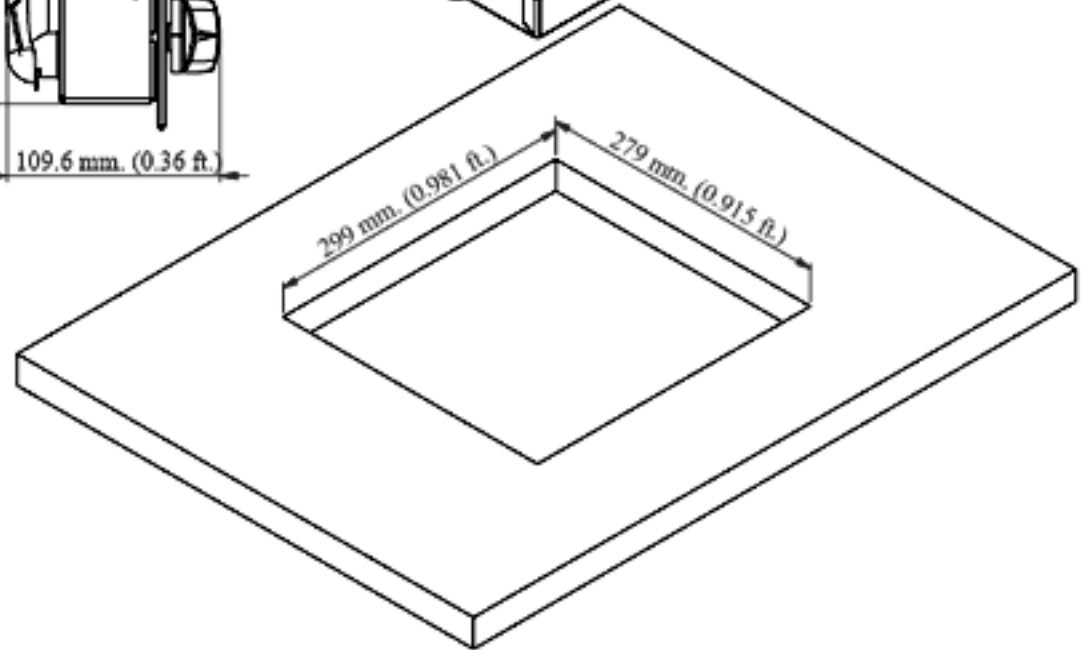
BUILT-IN DIMENSIONS
