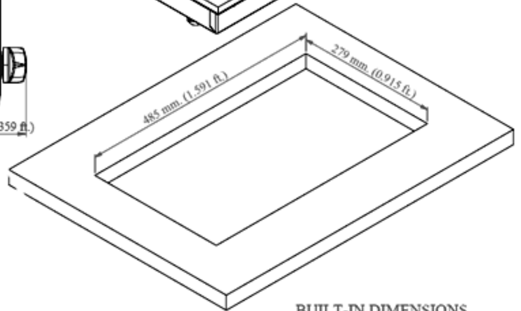
BUILT-IN DIMENSIONS
